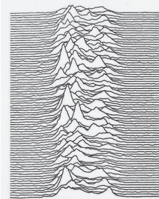
6.7: Successive pulses from the first pulsar discovered, CP 1919, are here superimposed vertically. The pulses occur every 1.332 seconds. They are viewed here rapidly-spinning around star.
